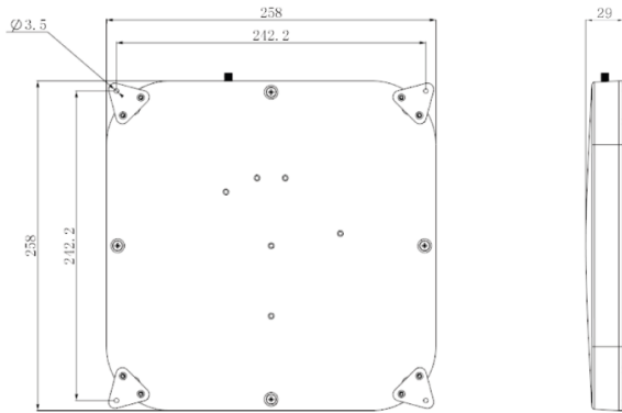
ATID-XC-AF812-D Type antenna appearance dimension drawing
